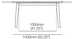
Side View Table Top Extension Stowed Under
