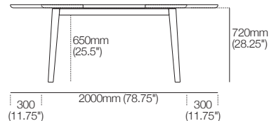
Side View Table Top Extended
